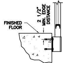
① FASCIA MOUNT
