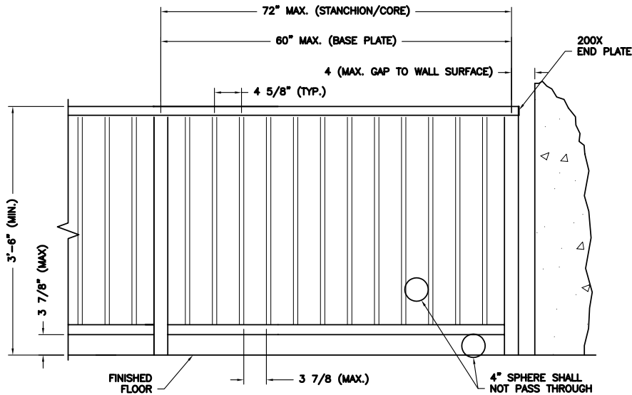
① TYPICAL ELEVATION
