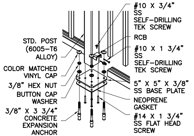
○ SURFACE MOUNTING DETAIL
