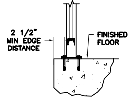
① SURFACE MOUNT
