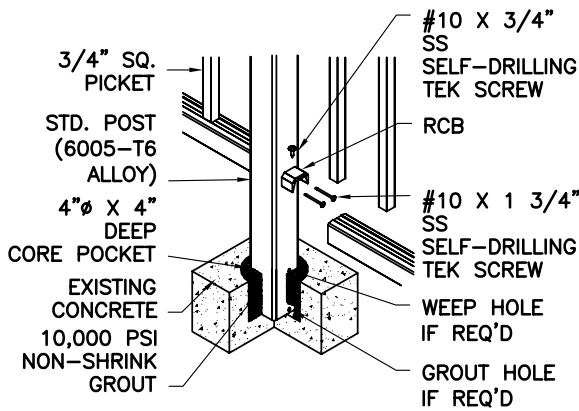
○ POST ONLY CORE POCKET DETAIL
