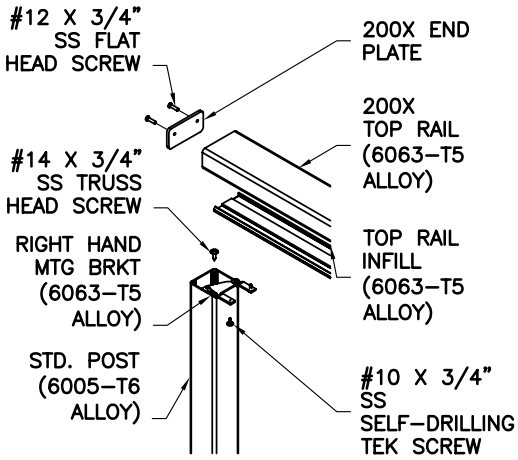
○ END CONDITION DETAIL
