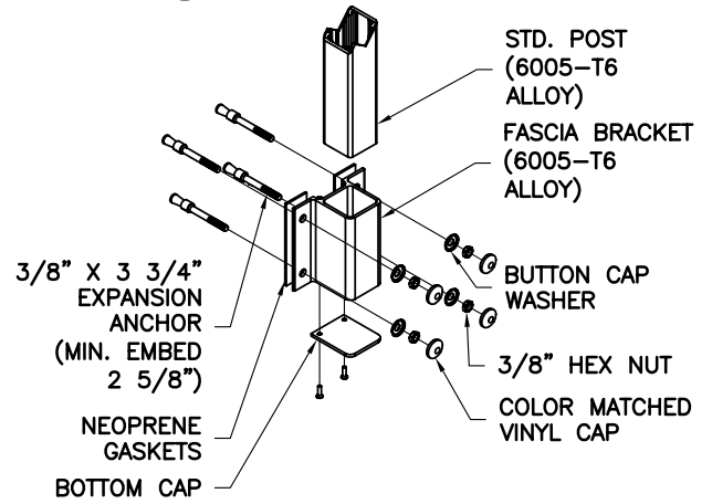
○ FASCIA MOUNTING DETAIL
