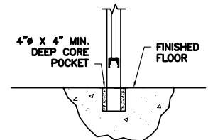
① CORE MOUNT
