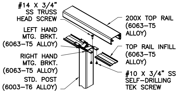
○ TYP. TOP RAIL CONNECTION
