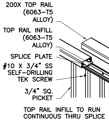
○ SPLICE PLATE DETAIL
